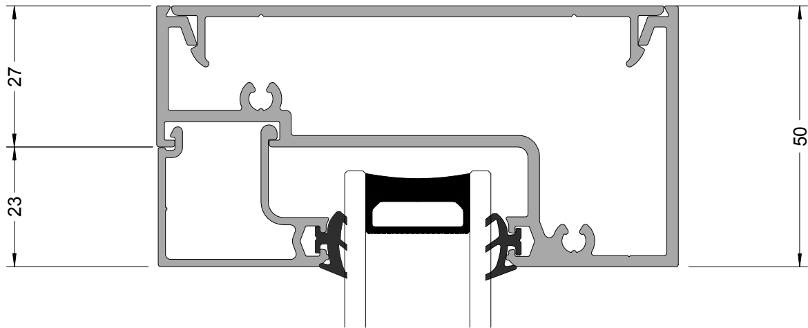
Fixed Frame
